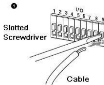
Figure 8-4 Install cable
