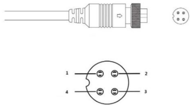
Figure 2-9 HDCVI aviation connector
