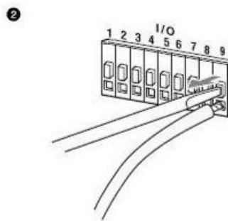
Figure 8-5 Remove cable
