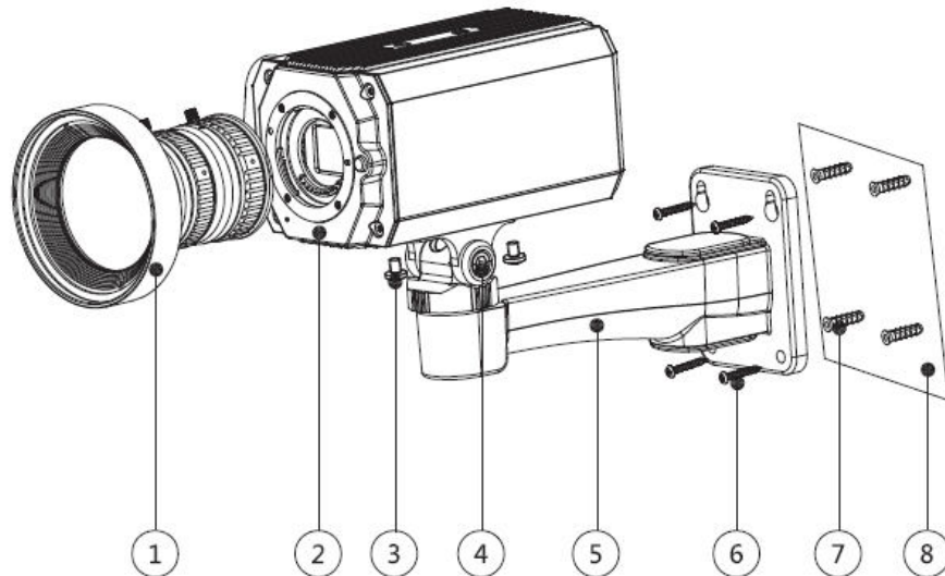
Figure 8-6 Device components
